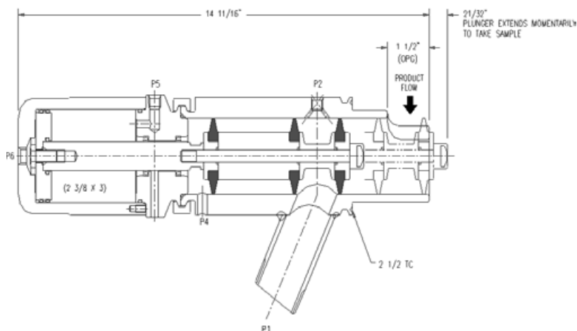
ISOLOK® SERIES SAH SAMPLER
