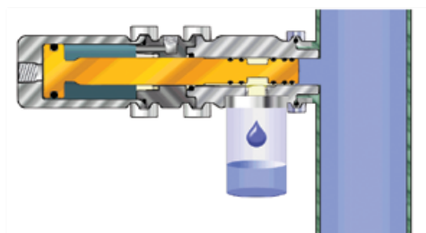
PLUNGER RETRACTED; SAMPLE ISOLATED AND LOCKED
