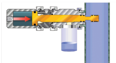
PLUNGER EXTENDED; PROCESS ISOLATED
